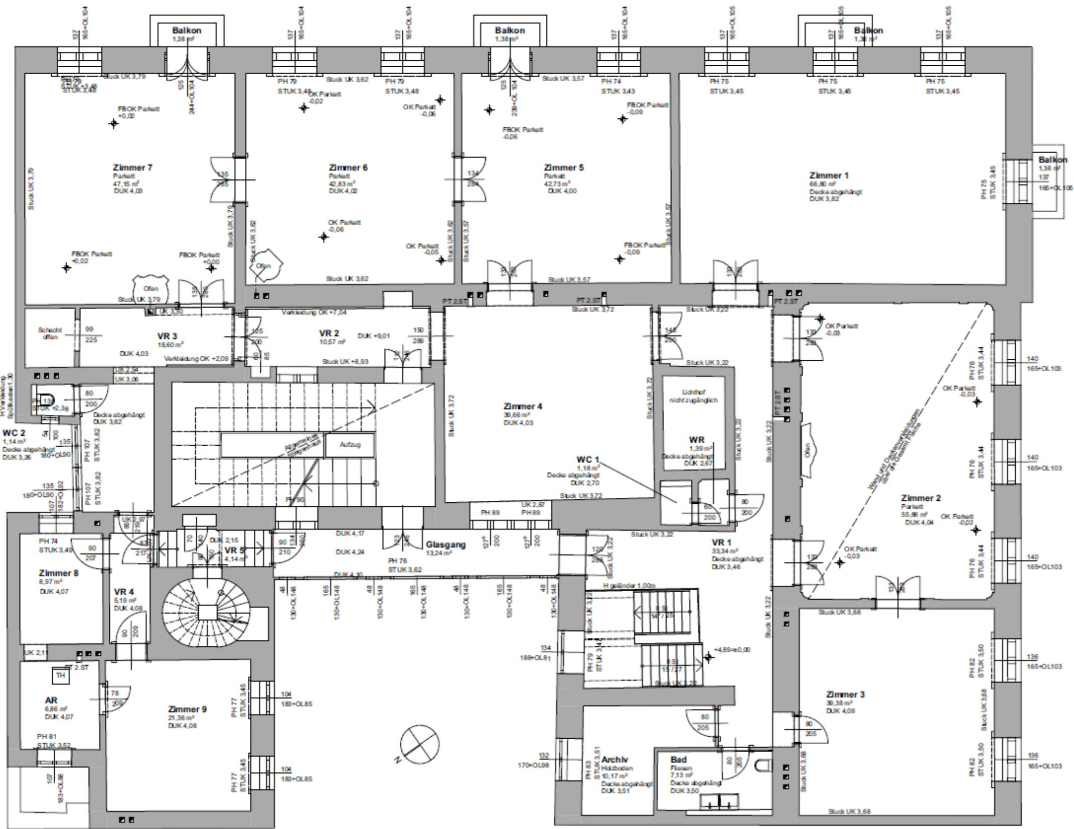
Grundriss 2. Stock
