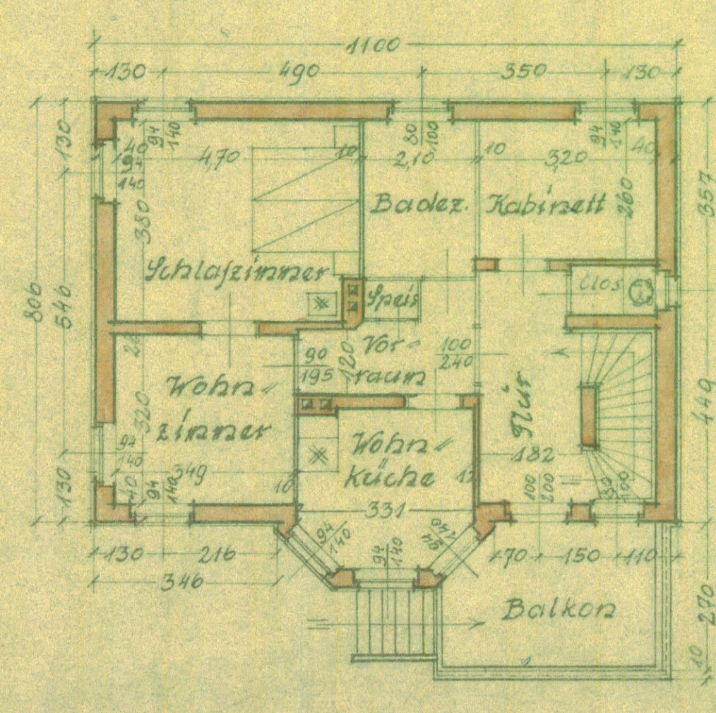
Grundriss 1. Stock
